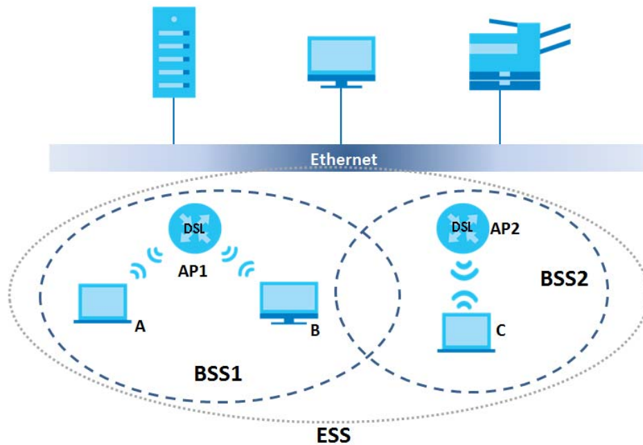
Figure 180 Infrastructure WLAN
