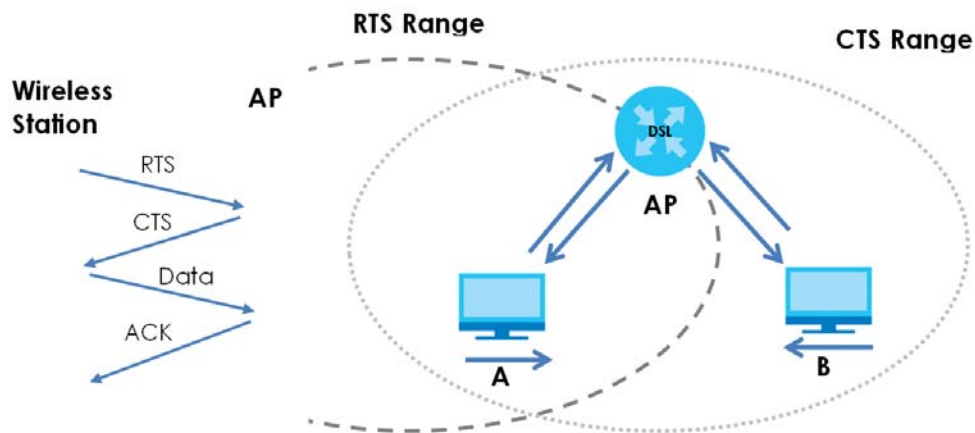
Figure 181 RTS/CTS
